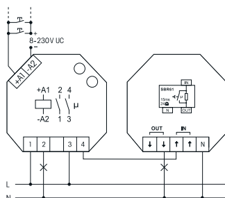
ESR61M-UC with SBR61-230V/120µF
