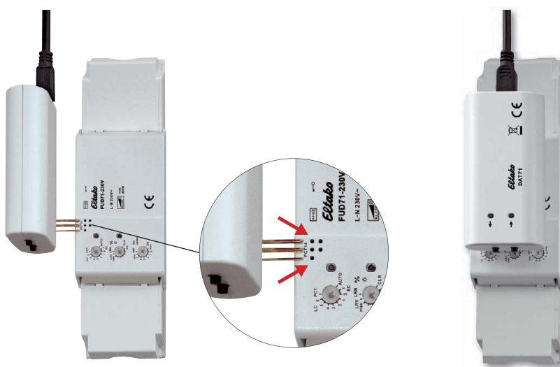
Plugging the data transformer DAT71 to a Series 71 actuator.
