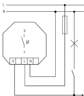
monitored circuit
