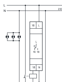
Control of emergency light systems via electric contactor I > 16 A ⚡ Emergency light systems with own battery supply
