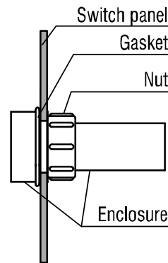
Fig. 5.4 Mounting
