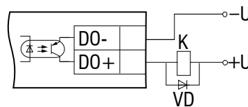
Fig. 5.7 NPN transistor output
