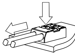
Fig. 5.3 Disconnecting the wire
