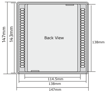
Fixing apparatus
